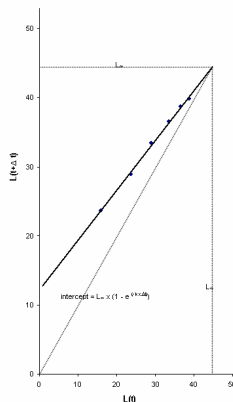
Fig 2: Ford-Walford plot for estimating L ∞ for Oreochromis niloticus at Gbedikere Lake, Kogi State.
