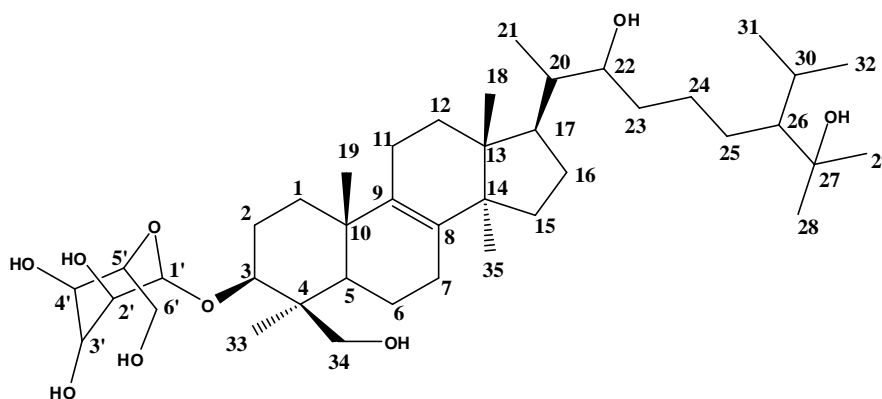
Figure 2: Chemical structure of compound 5
