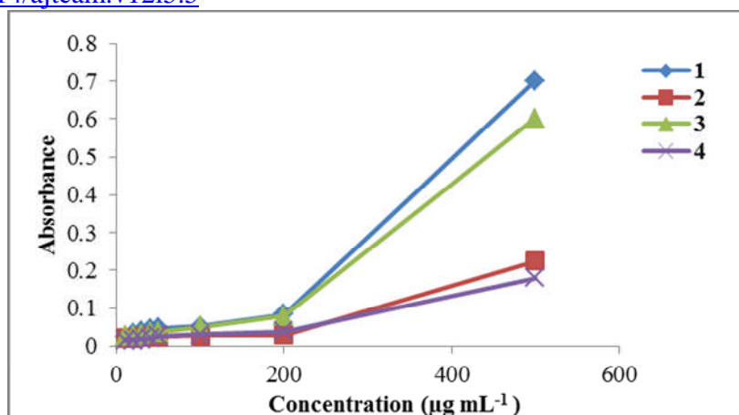
Figure 3: Comparison of the ferric reducing/ antioxidant power of compounds 1-4
