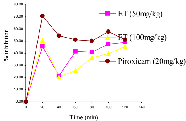
Fig. 2: Percentage inhibition of ET of P. kotschyii and Piroxicam on raw egg albumin-induced oedema in Rat
