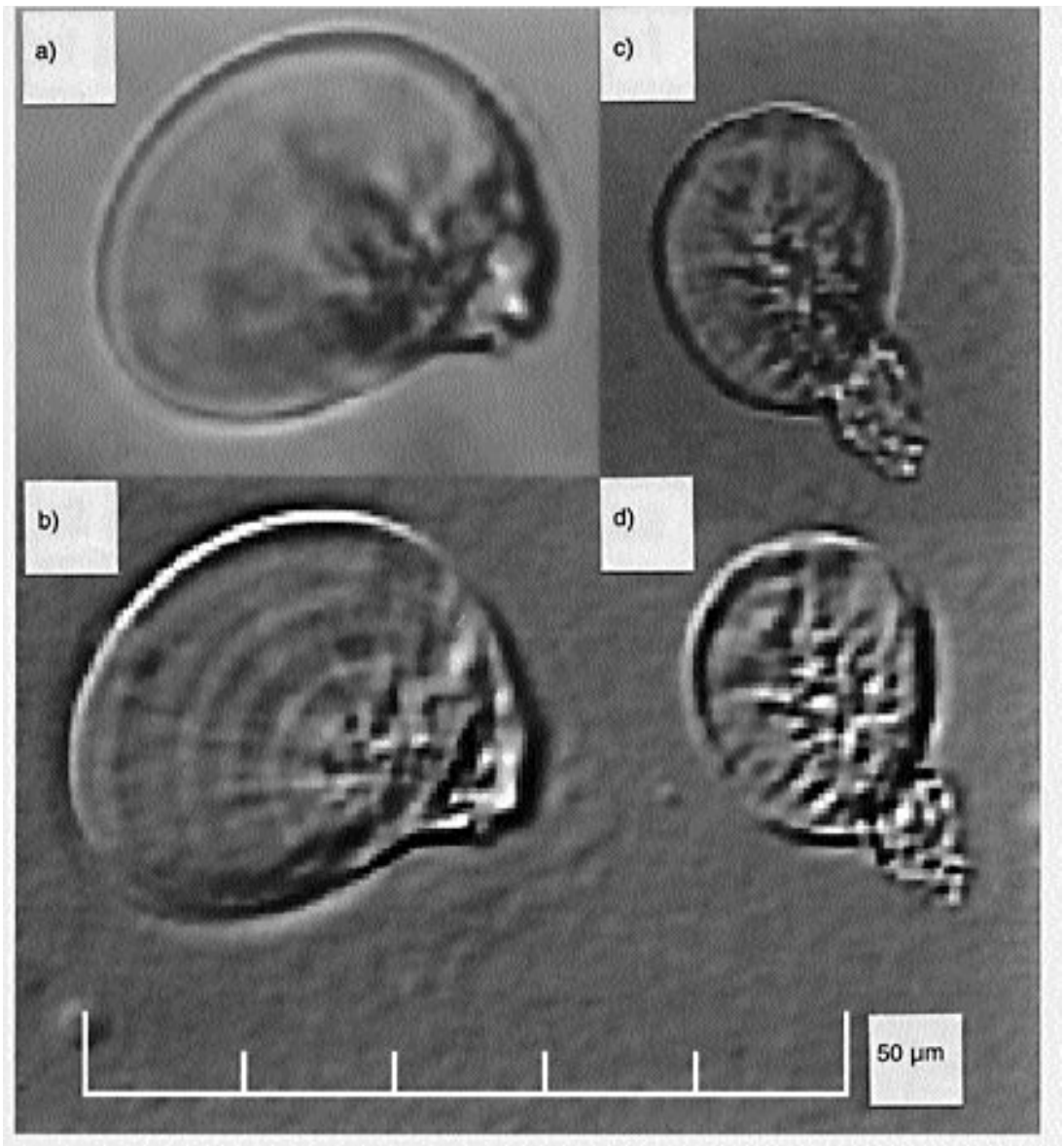
Fig. 5: Statoliths from laboratory-reared Illex argentinus hatchlings. (a) Raw image, statolith extracted from a Stage 30 hatchling of 1.54 mm ML ; (b) edge-enhancement-filtered image applied to (a); (c) raw image, statolith extracted from a Stage 28 hatchling of 1.32 mm ML ; (d) edge-enhancement-filtered image applied to same panel of (c)
