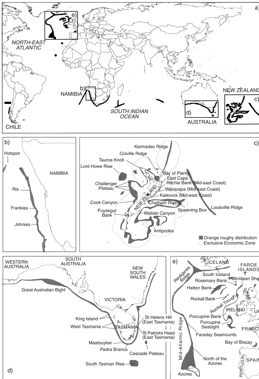
Fig. 1: Distribution of orange roughy (a) worldwide, with insets of the distribution (b) off Namibia, (c) around new Zealand, (d) around Australia, and (e) in the North-East Atlantic. Primary sources – Kotlyar (1996), Branch (1998), Magnússon and Magnússon (1998), Clark (1999, 2001), Gordon (1999), Tracey and Horn (1999), Bax (2000), Strutt (2000), Anderson (2001), Hareide and Garnes (2001), Hope (2001)
