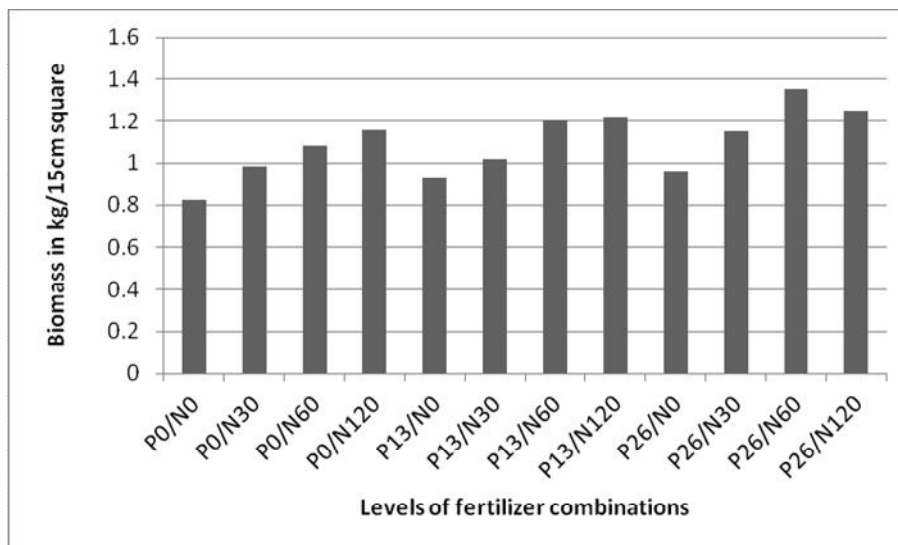
Figure 3: Means of all varieties on P and N fertilizer combination of dry shoot biomass yield/15 cm 2 quadrant for two years (L.S.D. = 0.156 and df of 119).
