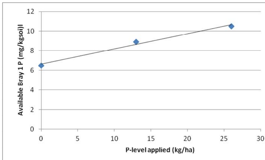
Figure 2: Available P measured as Bray 1 P upon application of P fertilizer (soils taken at 0-20cm two weeks after application at soil water capacity of 20% W/V)
