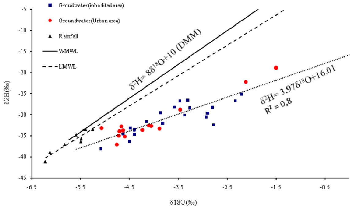
Figure 7. 18 O versus Deuterium ( 2 H) plots of rainwater and groundwater (March 2007).
