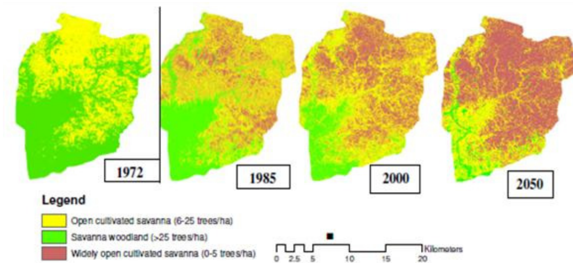
Figure 2. Land use and land cover maps of 1972, 1985, 2000 and 2050 in the savanna zone.
