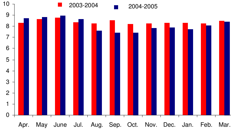
Figure 8. showing monthly variations in pH of water.
