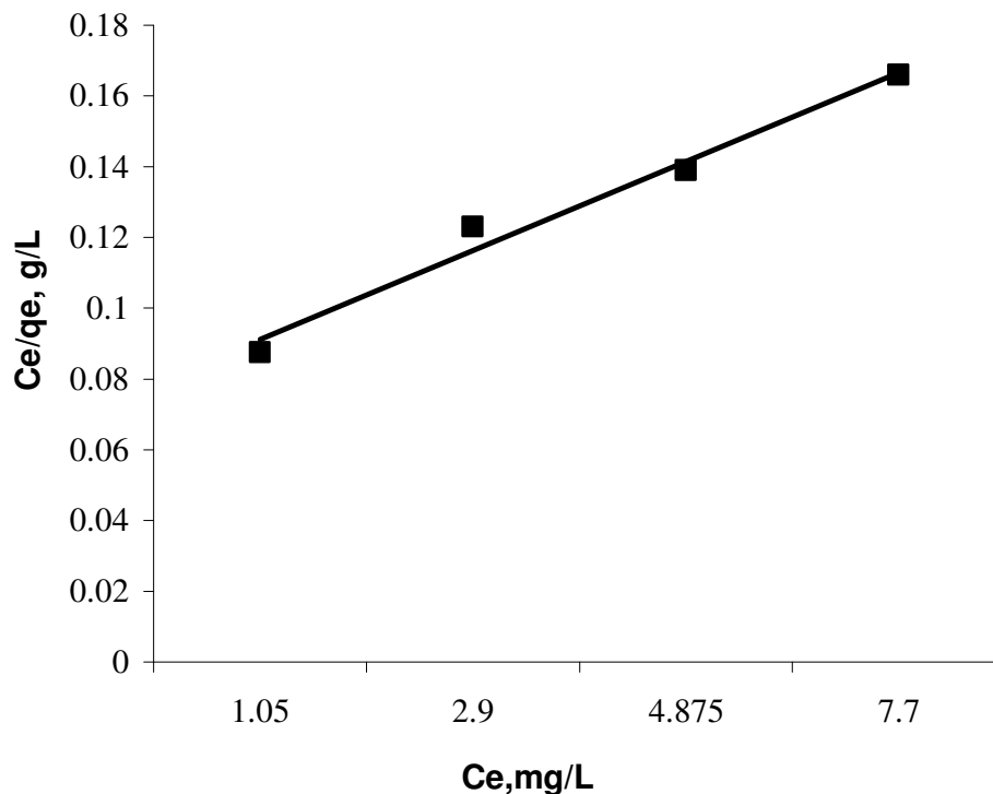
Figure 3. Langmuir plot for Congo red sorption onto water hyacinth roots. (M, 0.1 g; V, 50 ml; pH, 6; temperature, 30 °C).
