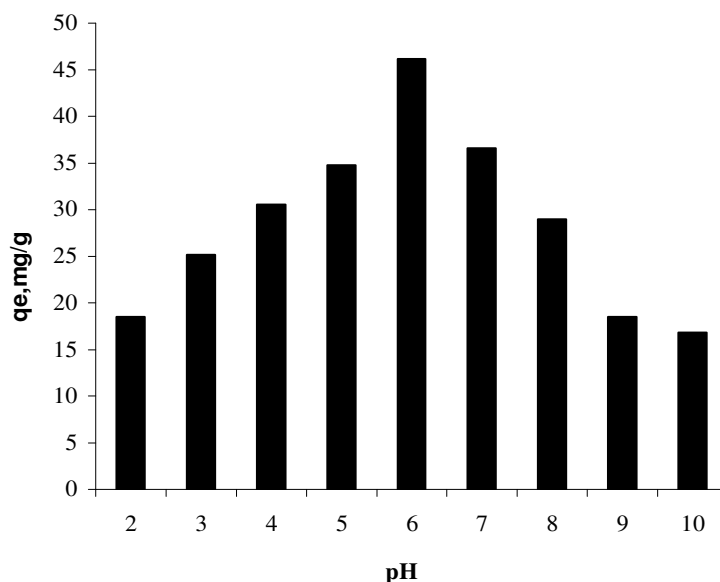
Figure 1. Effect of pH on equilibrium uptake of Congo Red (M, 0.1 g; V, 50 ml; Co, 100 mg/l; temperature, 30 °C)
