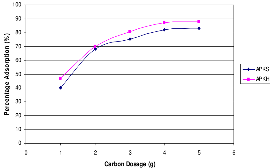
Figure 6. Plot of carbon dosage against percentage lead adsorption with APKS and APKH.
