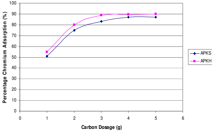
Figure 5. Plot of carbon dosage against percentage chromium adsorption with APKS and APKH.
