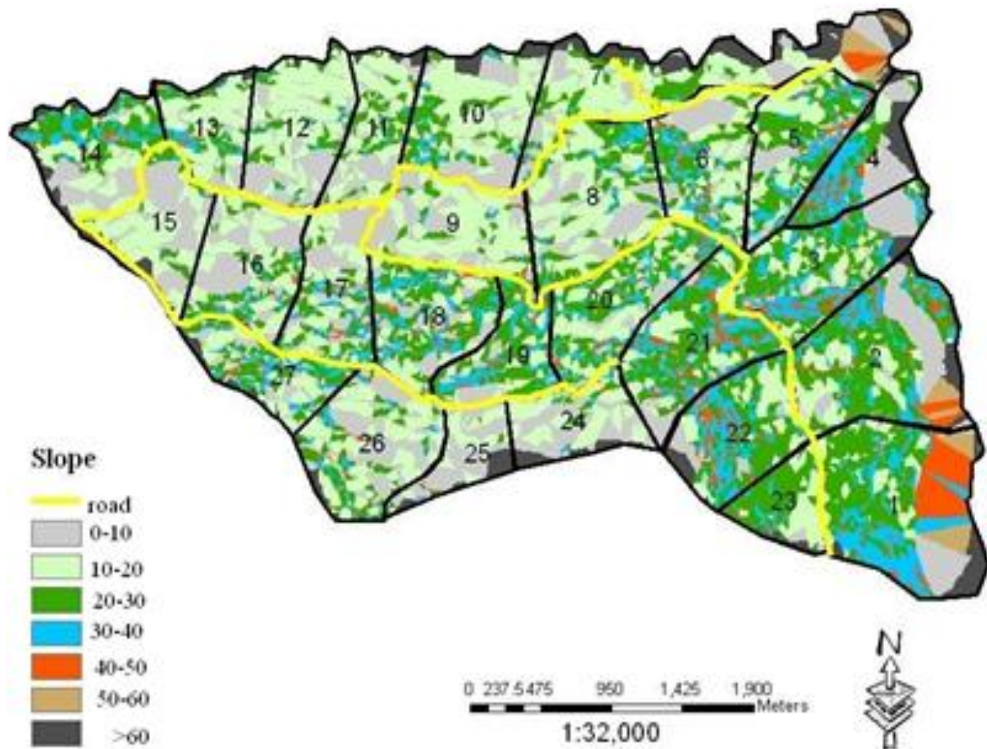
Figure 3. The map of slope classes in study area.
