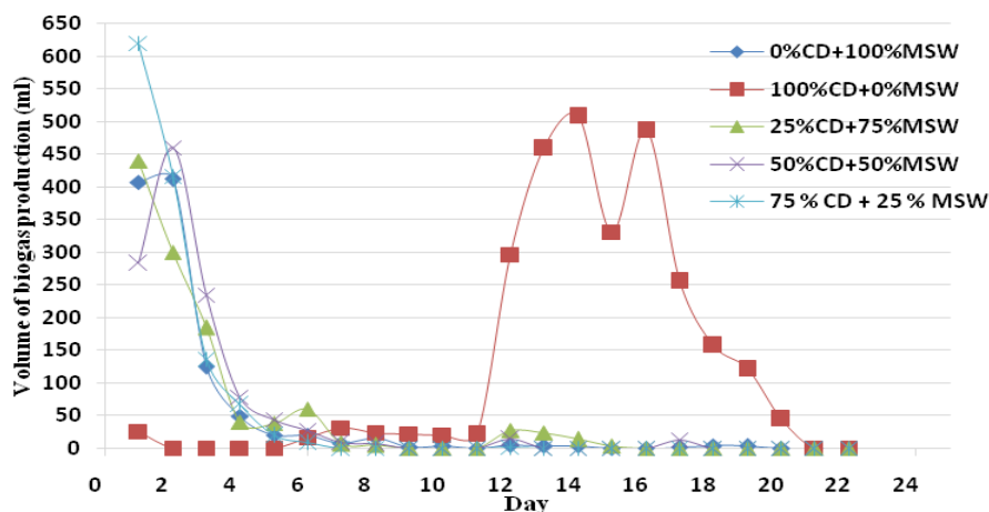
Fig. 4: Biogas yield of different substrate combinations
