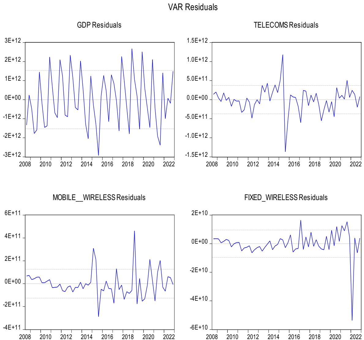
Figure 4.3: VAR Residual Graphical Residual Test
