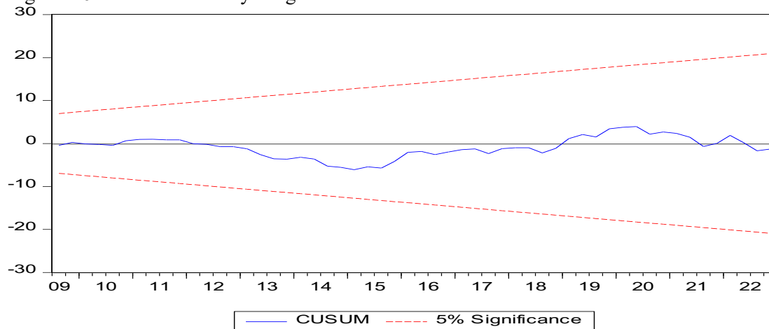
Figure 4.6: CUSUM Stability Diagnostics Test
