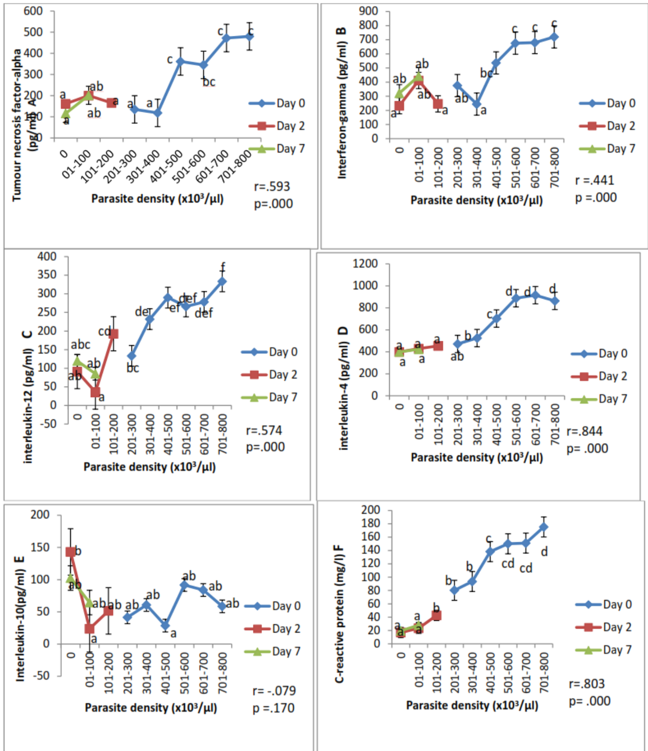
Figure 2: Responses of selected inflammatory markers to change in parasite density in children with severe malaria before, during and after treatment with artesunate/artemether-lumefantrine combination therapy.
