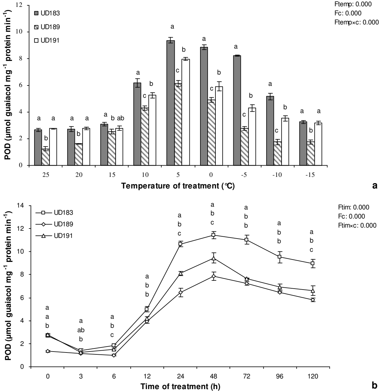
Figure 7. Activities of peroxidase (POD) in the cuttings of three poplar hybrid clones exposed to (a), different temperatures for 24 h; and (b), low temperatures (5°C) for different periods. The data presented are means ± SE (n = 5). Lowercase letters refer to differences between the three hybrid clones at the same temperature (a), or time treatment (b). Values followed by letters are significantly different from each other at P < 0.05 according to Duncan's method. F temperature, the effect of the different temperature treatment; Fc, the effect of clones; Ftim, the effect of low temperature treatment for different periods; F temperature × c, the temperature × clones interaction effect; F tim × c, the time × clones interaction effect, as determined by ANOVA.
