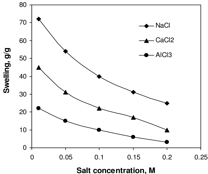
Figure 7. Swelling capacity of hydrogels in salt solutions (0.15 mol/L).
