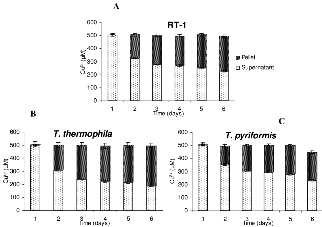
Figure 9. Uptake of copper ions by Tetrahymena RT-1 (A), T. thermophila (B) and T. pyriformis (C) from the Bold-basal salt medium containing 500 \mu\text{M} copper supplemented with 0.1% glucose at 28 \pm 2^\circ\text{C} and pH 7.2. There is gradual decrease in concentration of copper ions in the medium with concomitant increase in the pellet, over a period of six days.
