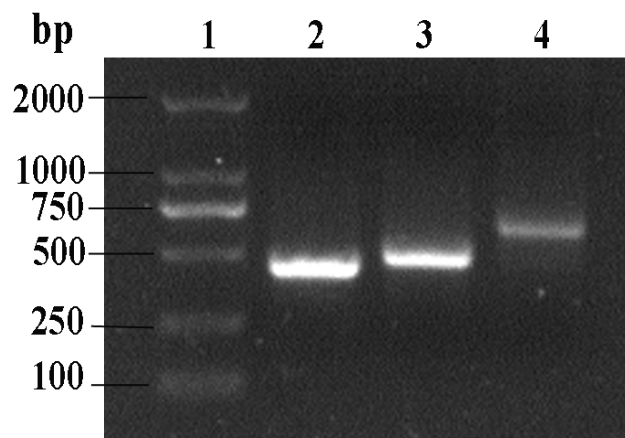
Figure 1. Identification of the products of RT-PCR, 3' RACE and 5' RACE. 1, DL2000 DNA marker; 2 to 4, samples from the product of 5' RACE, RT-PCR and 3' RACE, respectively.
