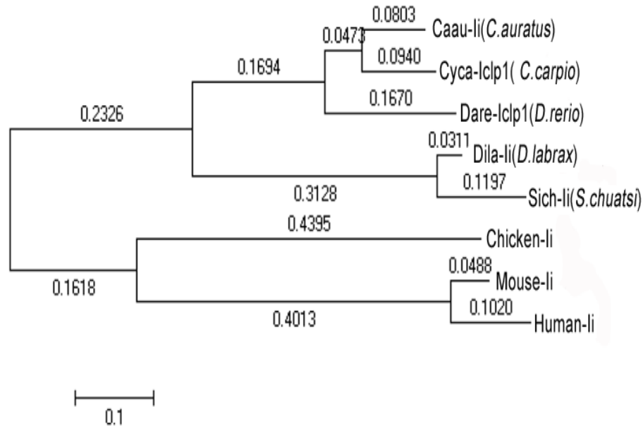
Figure 4. Neighbour-joining tree of li amino acid sequences generated by MEGA4 program.
