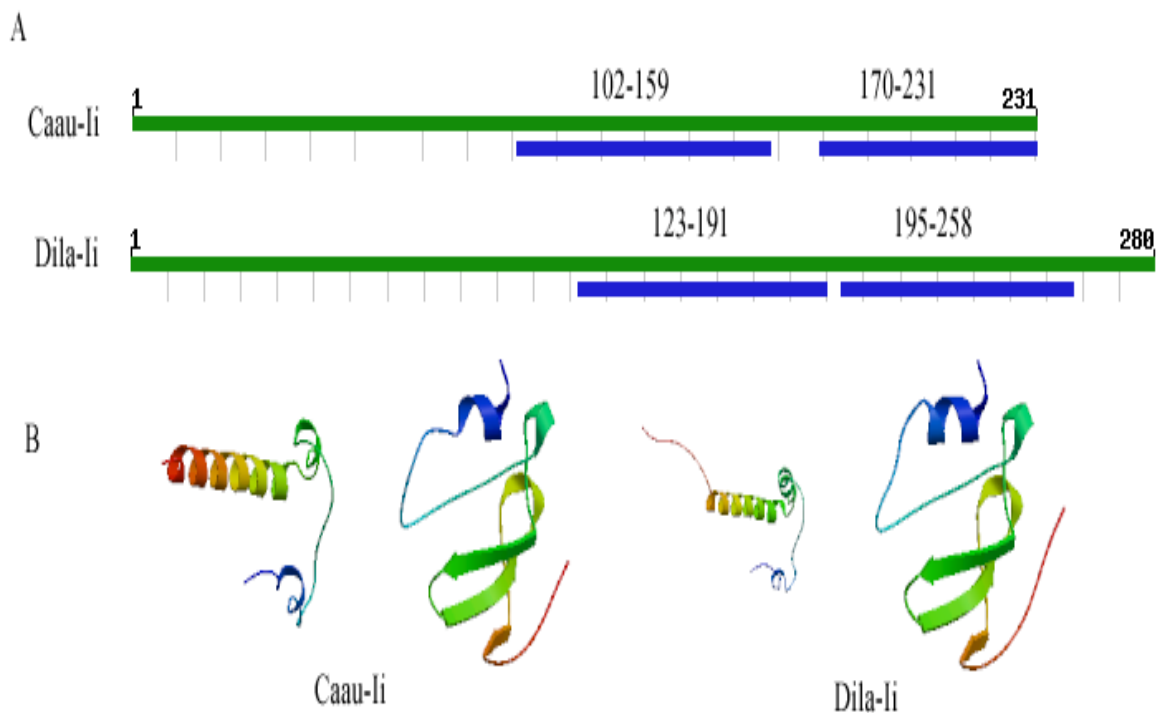
Figure 5. Homology modeling of the conformation of Caau-li ( C. auratus li) based on the structure of Dila-li ( D. labrax li). (A) There are two main domains of CLIP and TRIM; (B) space structure alignment of domains of Caau-li and Dila-li .
