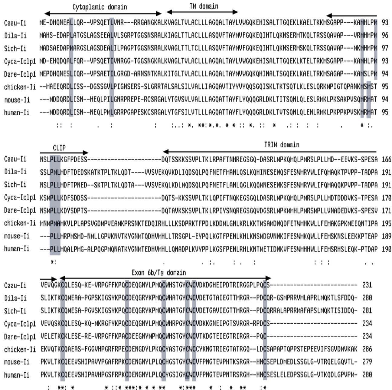
Figure 3. Alignment of C. auratus li cDNA with representative homologues of the li of other vertebrates. GenBank accession numbers not previously mentioned are: Cyprinus carpio (Cyca-Ic1p1), BAC53767; D. labrax (Dila-Ii), ABH09445; Siniperca chuatsi (Sich-Ii), AAS77256; Danio rerio (Dare-Ic1p1), AAD24542; Gallus gallus (chicken-Ii), CAC27415; Homo sapiens (human-Ii), P04233; Mus musculus (mouse-Ii), P04441. Different domains, including cytoplamic, TM (transmembrane), CLIP (class II-associated li-derived peptide), TRIM (trimerization) and Tg (thyroglobulin) structures, are indicated by arrows.
