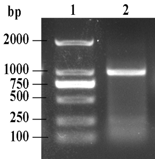
Figure 2. Identification of the PCR product of full-length Caau-li . 1, DL2000 DNA marker; 2, PCR product of full-length Caau-li .
