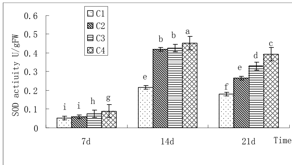
Figure 3. Superoxide dismutase activity of C. demersum . C1, Oligotropher; C2, mesotropher; C3, eutropher; C4, hypertrophic.
