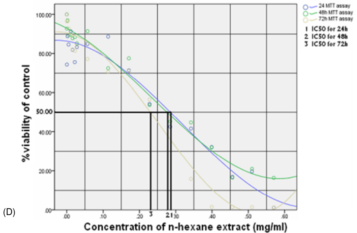
Figure 2. Cytotoxic effect of n-hexane extract on A549 lung cancer cell line after 24 h (A), 48 h (B) and 72 h (C) exposure. (D). IC50 of n-hexane extract of Curcuma longa on A549 tumor cell line after 24, 48 and 72 h treatment.
