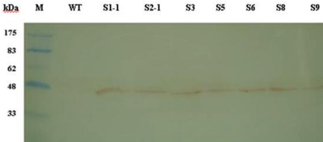
Figure 1. Western blot analysis of the ZmPti1 gene expression in wild type Arabidopsis plants and seven ZmPti1 homozygous transgenic lines. M, protein molecular weight marker; WT, wild type Arabidopsis ; seven transgenic lines: S1-1, S2-1, S3, S5, S6, S8, S9.
