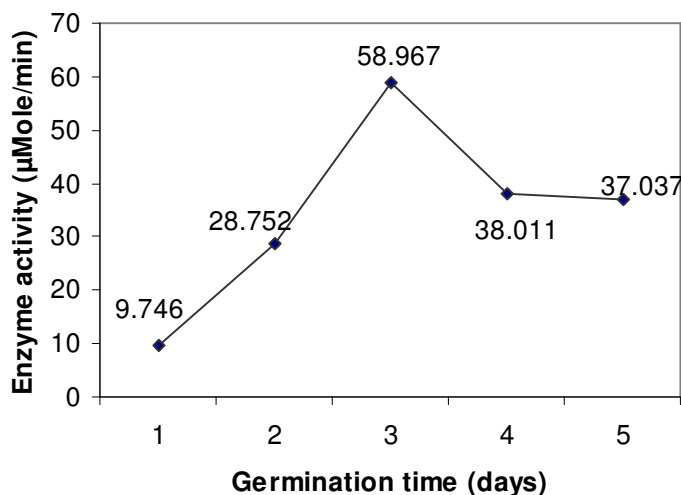
Figure 4. Effect of germination on the activity of corn α-amylase.
