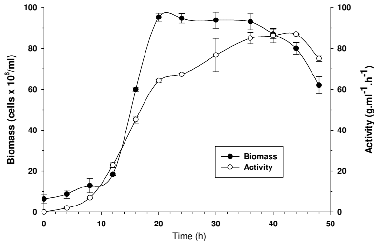
Figure 2. Time course of cell growth and amylase production of strain Ba3.
