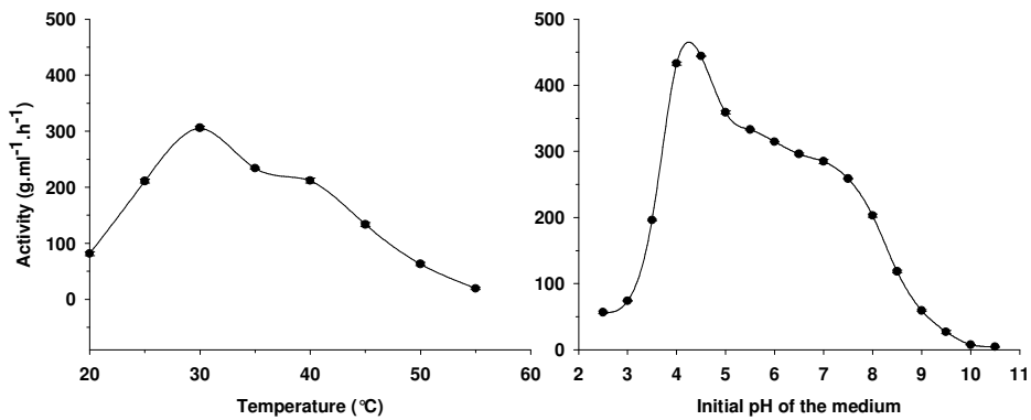
Figure 3. Effect of temperature and initial pH of the medium on amylase production.
