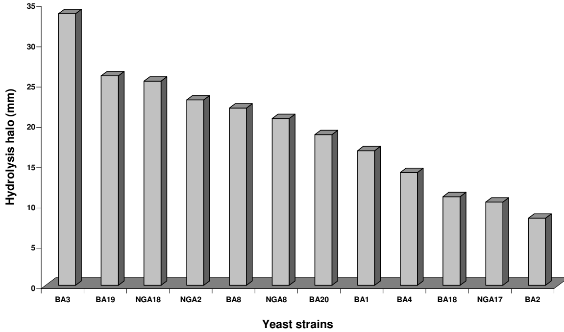
Figure 1. Amyolytic activity of isolated yeast strains after 48 h fermentation at 30°C.
