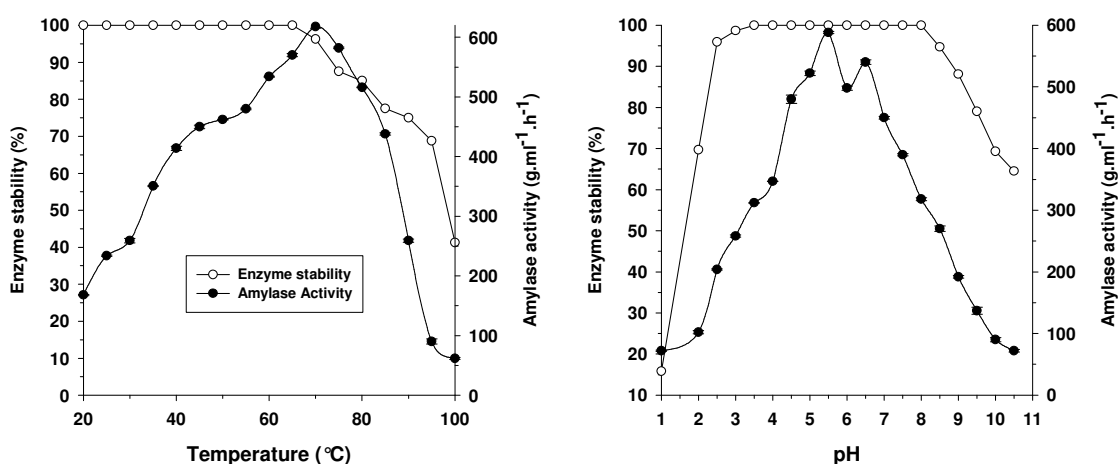
Figure 4. Effect of temperature and pH on the enzyme activity and stability.
