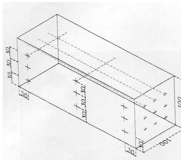
Figure 1. Measuring points of inner compost temperature
