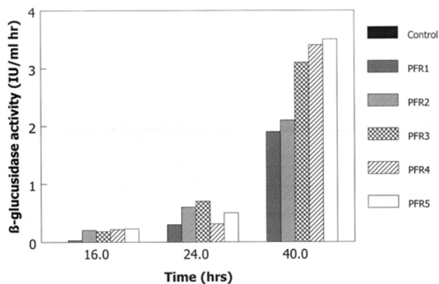
Figure 2. Production of beta-glucosidase by bombarded yeast harbouring chromosomal DNA from C. biazotea restricted with SacI grown on 1% cellulobiose after 40 h.
