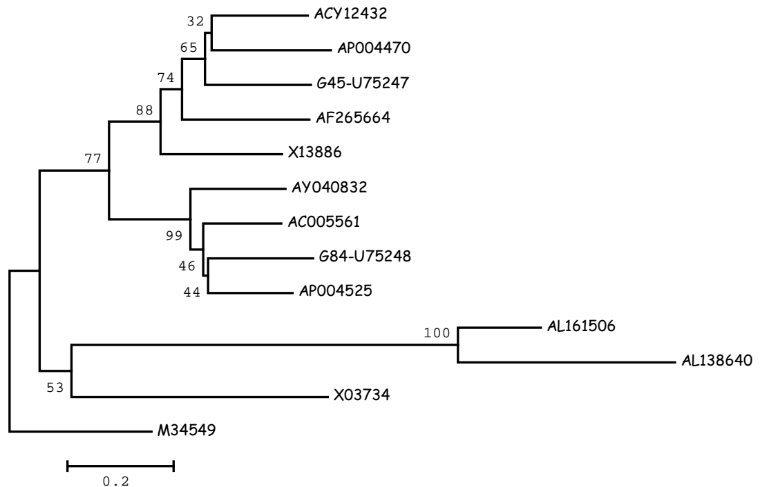
Figure 2. Phylogenetic tree showing relationship between reverse transcriptase nucleotide sequences of G. barbadense G45 and G84 and plant gypsy retrotransposons. The Neighbour-Joining method (Saitou and Nei, 1987) was used to construct the tree. The numbers on the branches represent bootstrap support for 1,000 replicates. Names refer to the accession number of the nucleotide sequences that encode the corresponding reverse transcriptase genes. Sequences used and their GenBank accession numbers include: ACY12432 Ananas comosus gypsy group retrotransposon (Thomson et al., 1998); AP004470 Lotus japonicus genomic DNA Chromosome 4 27319-27627 (Sato et al., 2001); AF25664 Solenum tuberosum resistance gene cluster 130667-130975 (Vossen et al., 2000); X13886 L. henryi del gypsy group retrotransposon (Smyth et al., 1989); X03734 Drosophila melanogaster gypsy retrotransposon (Yuki et al., 1986); AL161506 Arabidopsis thaliana Chromosome 4 182355-182050 (Marin and Llorens, 2000); AL138640 A. thaliana Chromosome 3 37138-36830 (Marin and Llorens, 2000); AC005561 Oryza sativa osr31/rir7 Ty3/gypsy LTR-retrotransposon (McCarthy et al., 2002); AP004525 L. japonicus genomic DNA Chromosome 5 65809-66114 (Sato et al., 2001); AY040832 Hordeum vulgare gypsy group retrotransposon cereba (Hudakova et al., 2001), and M34549 yeast Ty3 retrotransposon (Hansen et al., 1986).
