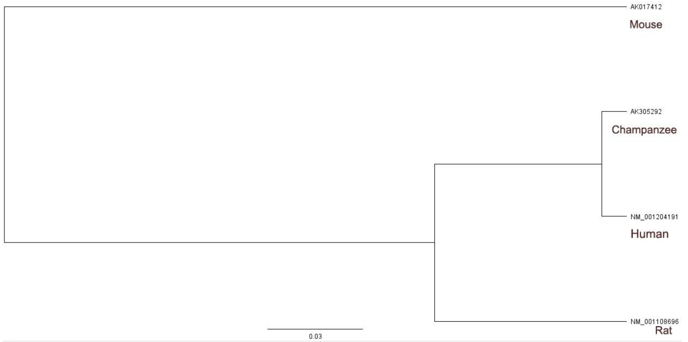
Figure 2. Phylogenetic analysis of nucleotide sequences.
