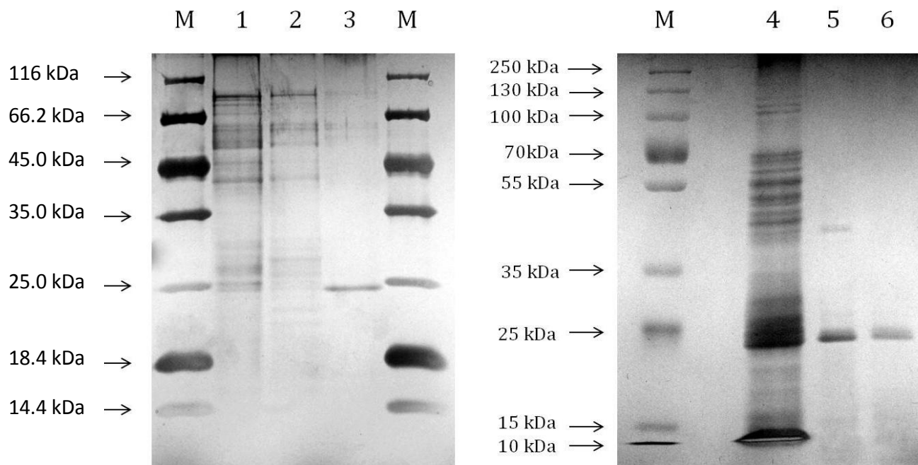
Figure 2. SDS-PAGE of post-cultivation broth proteins from D. geothermalis in the fraction during purification steps. M, Molecular weight marker; 1, fraction precipitated at 30% (\text{NH}_4)_2\text{SO}_4 saturation; 2, fraction precipitated at 45% (\text{NH}_4)_2\text{SO}_4 saturation; 3, fraction precipitated at 90% (\text{NH}_4)_2\text{SO}_4 saturation; 4, post-cultivation broth; 5, fraction precipitated at 90% (\text{NH}_4)_2\text{SO}_4 saturation; 6, fraction after gel filtration.
