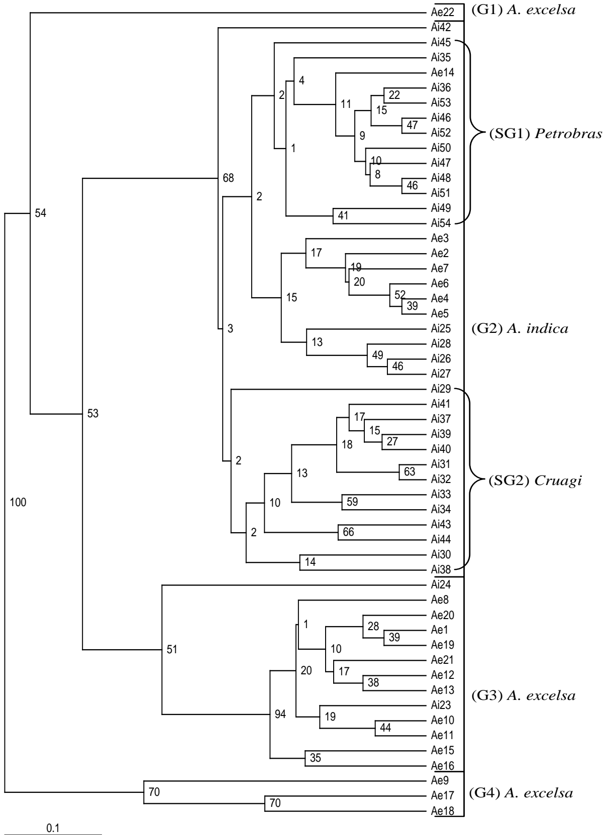
Figure 4. Dendrogram of genetic similarity generated using the Jaccard coefficient and the UPGMA method with analysis bootstraps for 54 neem accessions ( Azadirachta sp.) belonging to Embrapa Coastal Tablelands (Araçaju, Sergipe, Brazil).
