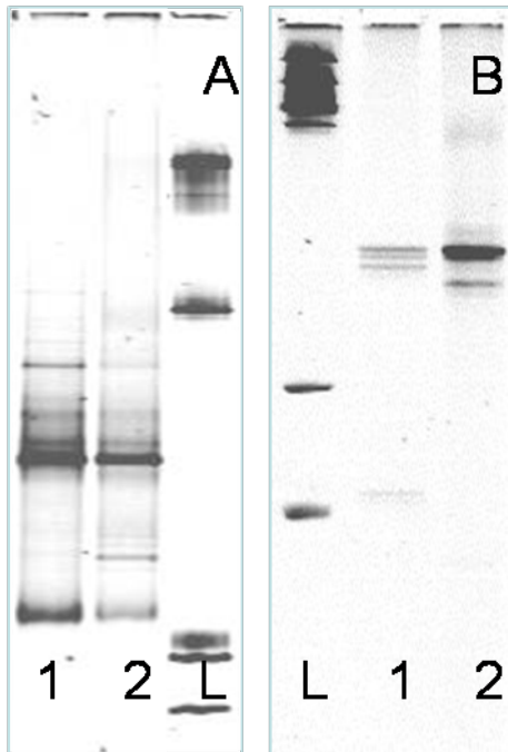
Figure 2. DGGE fingerprinting profiles of amplified V6 to V8 (A) and V3 (B) 16S rRNA genes regions obtained from extracted DNA from cheese samples from farms 1 (1) and 2 (2).
