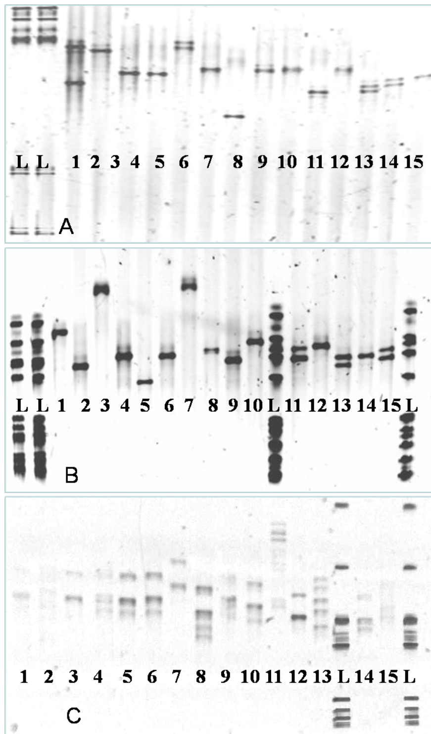
Figure 1. DGGE fingerprinting profiles of variable V6 to V8 (A), V3 (B) and V1 (C) 16S gene regions obtained from extracted DNA from 15 bacterial species. Lanes 1, L. brevis ; 2, L. rRNA bulgaricus ; 3, L. gasseri ; 4, L. helveticus ; 5, L. paracasei ; 6, L. lactis ; 7, L. casei ; 8, L. lactis subsp. Lactis ; 9, E. faecium ; 10, E. faecalis ; 11, E. villorum ; 12, E. asini ; 13, E. maloduratus ; 14, E. durans ; 15, E. avium .
