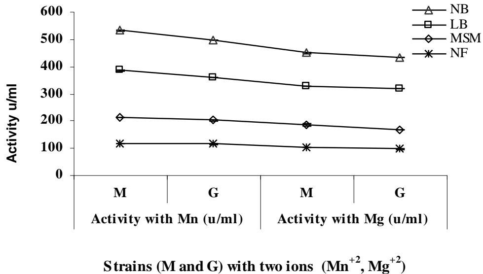
Figure 4. Effect of different media on GS activity from Paenibacillus polymyxa (M and G strains) with Mn^{+2} , Mg^{+2} ions.
