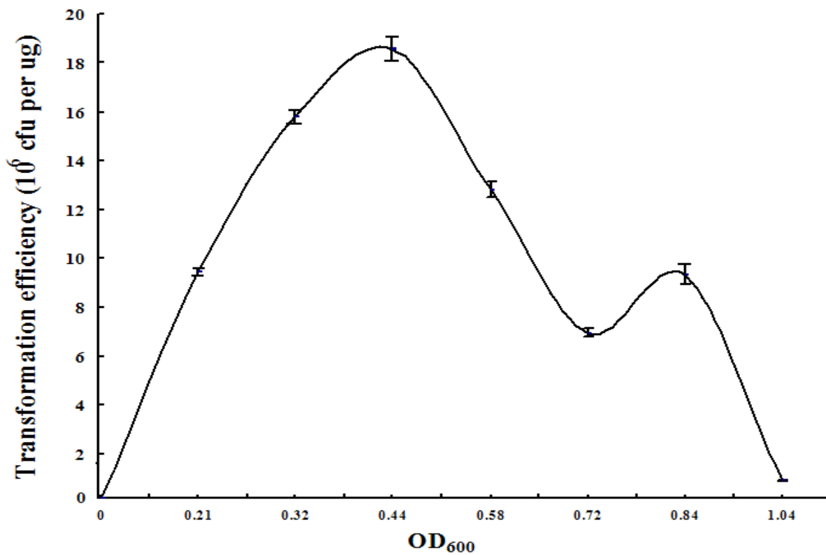
Figure 3. Average transformation efficiency of competent cells from different OD 600 value (from 0.2 to 1.0) Results shown are the average units for triplicate assays. Error bars represent standard deviation.
