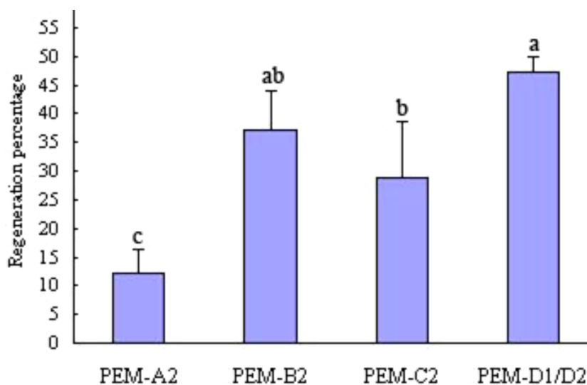
Figure 2. Average percentage of PEMs that developed into differentiated plantlets data were collected 4 weeks after the PEMs were transferred to light. Means with the same letter are not significantly different from each other at p=0.05 .
