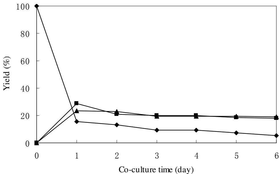
Figure 1. Time-course of biotransformation of dihydro-epi-deoxyarteannuin B (1) by the suspension-cultured cells of A. carambola . Yields of 1 (◆), 2 (■), 3 (▲) are plotted.
