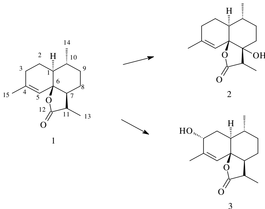
Figure 2. Proposed biosynthesis pathways of dihydro-epi-deoxyarteannuin B (1) by the suspension-cultured cells of A. carambola .
