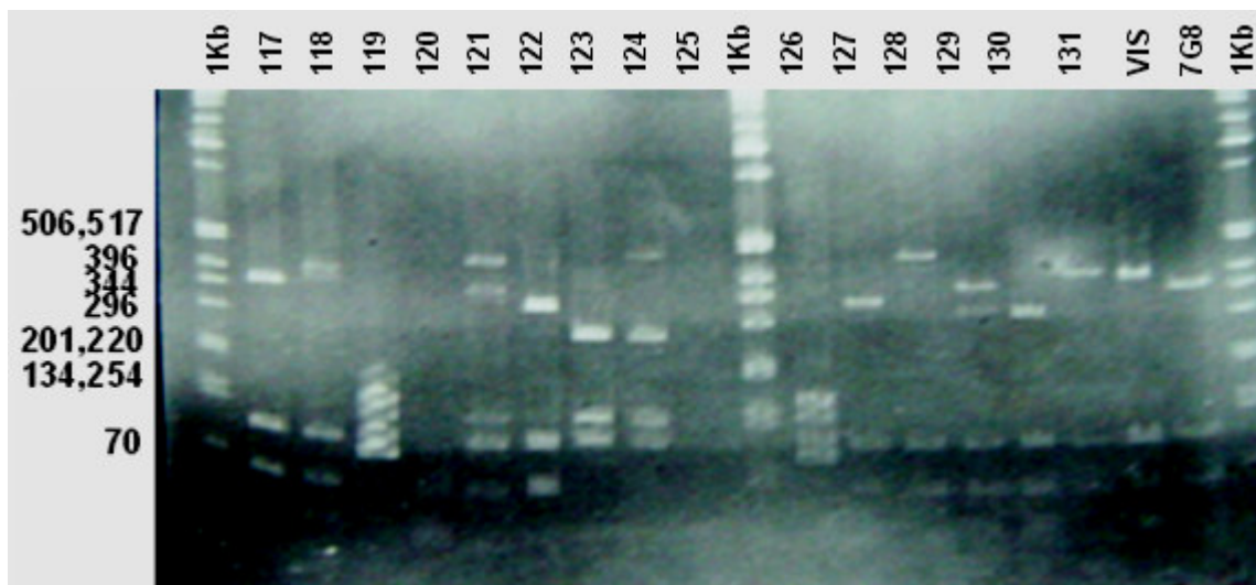
Figure 3. MSP2 RFLP products on 10% PAA gel. Lanes 122 and 123 represent the 3D7 and FC27 allelic families, respectively. The patterns of fragment sizes are 70, 108, 290 bp for 3D7 and 115, 137, 260 for FC27 in that order. Lanes 119 and 126 indicate degraded DNA fragments.
