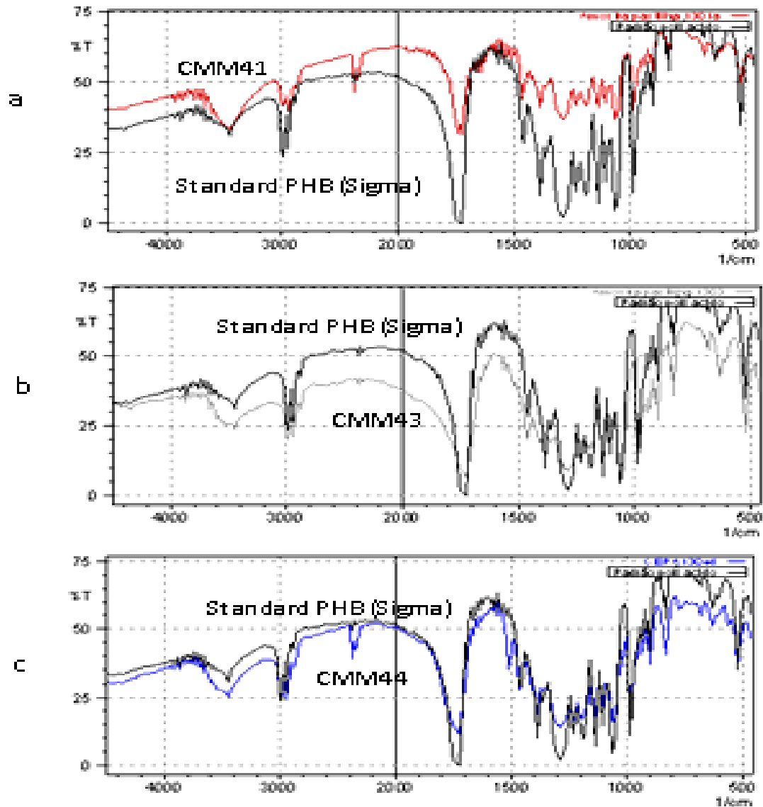
Figure 2. FTIR spectra of the polymers from strains (a) CMM41, (b) CMM43 and (c) CMM44 compared to the PHB standard.
