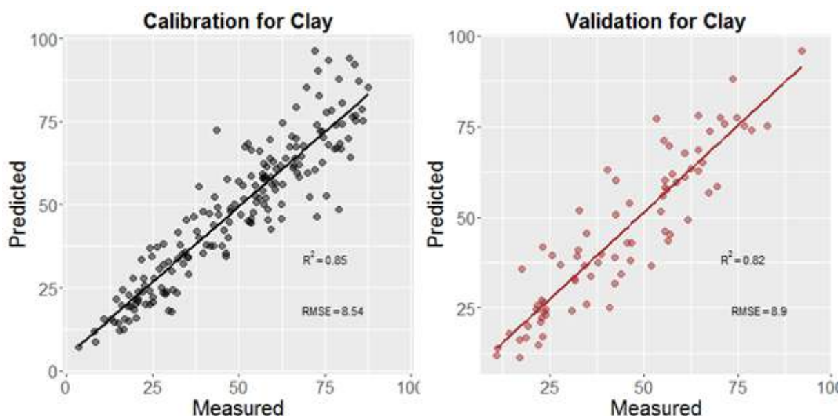
Figure 4: Calibration and validation of partial least squares model developed to predict clay content of soil (g clay kg -1 soil; n calibration =182 samples; n validation =78 samples).
