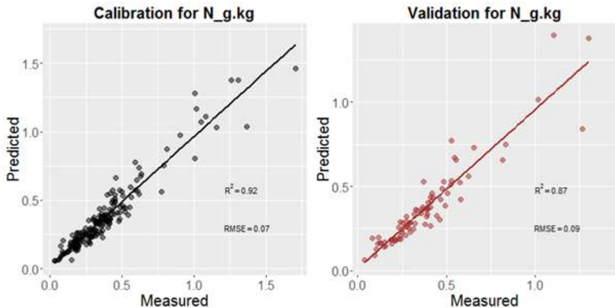
Figure 3: Calibration and validation of partial least squares model developed to predict the total N concentration of soil (g N kg -1 soil; n_{\text{calibration}}=182 samples; n_{\text{validation}}=78 samples).
