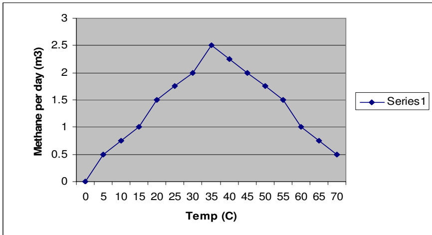
Fig. 2 Above: Methane production per day at varying temperatures in South-eastern Nigeria.
