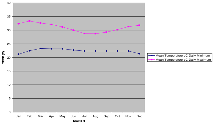
Fig.1: Temperature records in south-eastern Nigeria in 2006.
