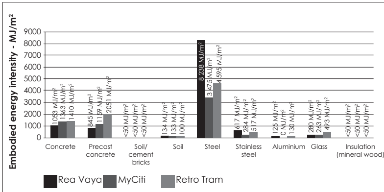
Figure 14: Comparison of embodied energy of specific materials
