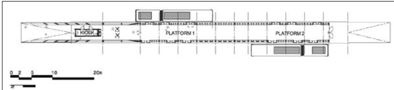
Figure 6: Plan of Switch station Source: Hugo, 2011: own plan
