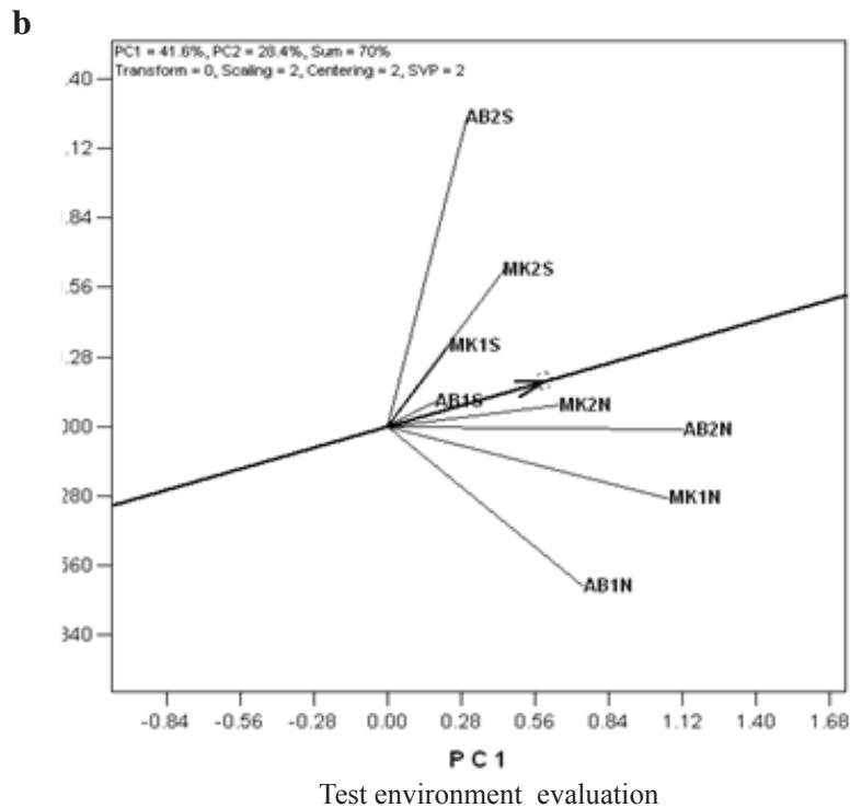
Figure 3. Average tester coordination view of the GGE biplot showing the discriminativeness and representativeness of the test environments (a) Evaluation of test locations across years; (b) Evaluation of test locations in each year. Abbreviations; MKS , Mokwa under Striga infestation, ABS, Abuja under Striga infestation, MKN, Mokwa under Striga -free conditions, ABN, Abuja under Striga -free conditions; 1 stands for year 2008 and 2 for 2009.
