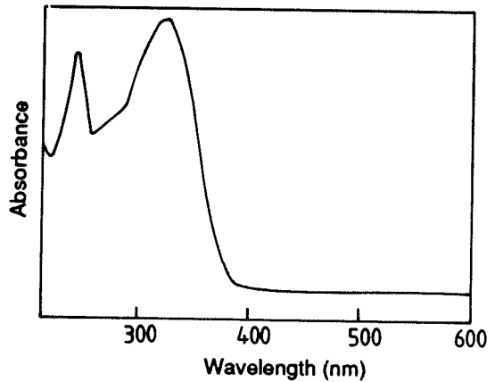
Figure 4. The UV spectrum of apigenin isolated from a tan plant. The spectrum was identical to that of standard apigenin ( \lambda_{\max} = 329 nm).
