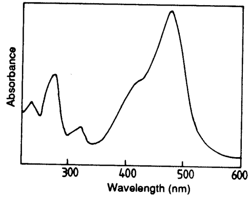
Figure 2. The UV-VIS spectrum of apigeninidin isolated from a red plant. The spectrum was identical to that of standard apigeninidin ( \lambda_{\max} = 475 nm)
