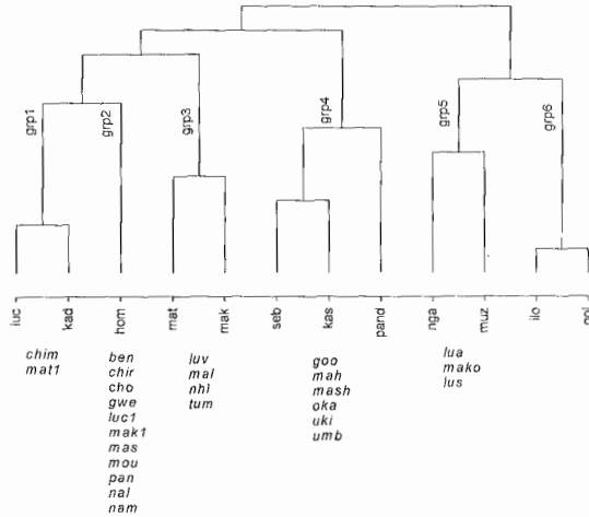
Figure 3. Dendrogram for cumulative classification of 38 sites in the SADC region based on grain yield per hectare of sorghum varieties planted during 1987/88 - 1992/93 and 1999/2000 using weighted environment-standardised squared Euclidean distance as dissimilarity measure and incremental sum of squares as clustering strategy.
